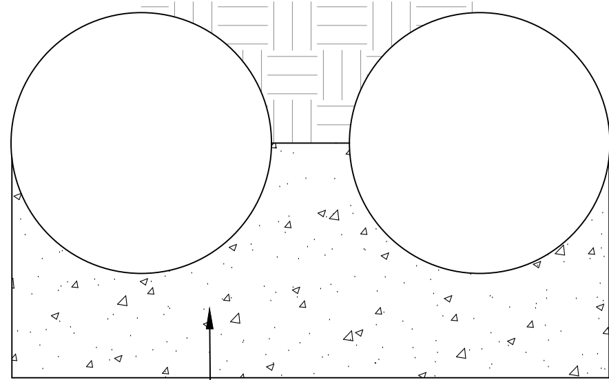
SIKA WATERTIGHT CONCRETE (min.200mm thickness)
