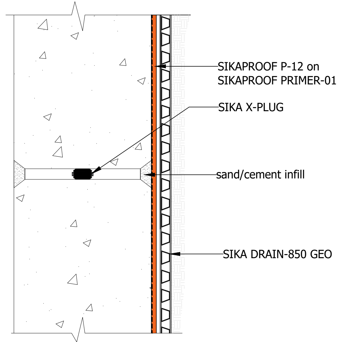
SIKAPROOF P-12 (Without Sleeve)
