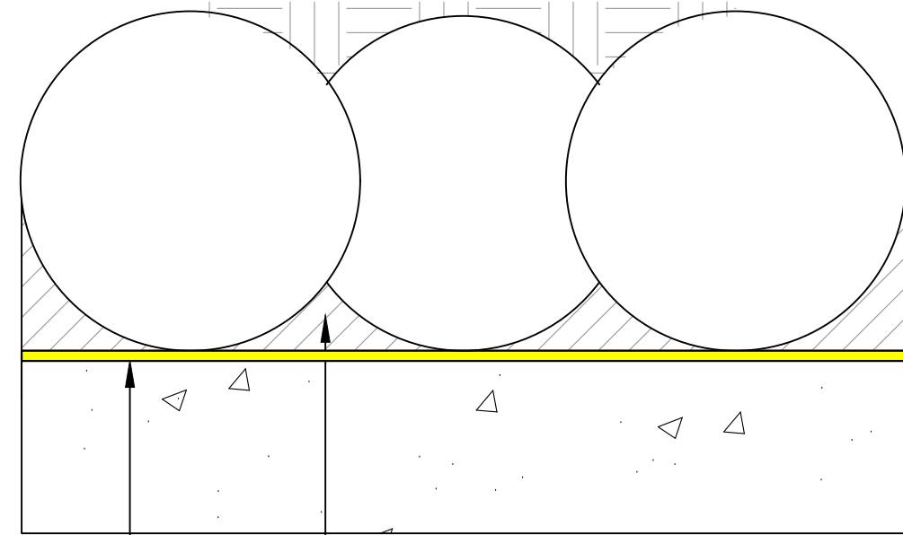
SIKAPROOF A sacrificial formwork/facing to pile
