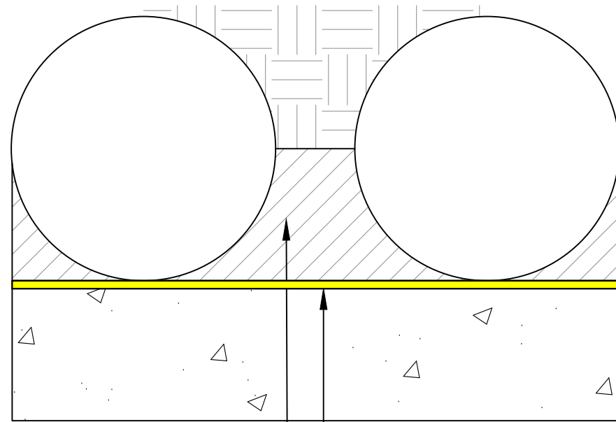
SIKAPROOF A back blinding/facing
