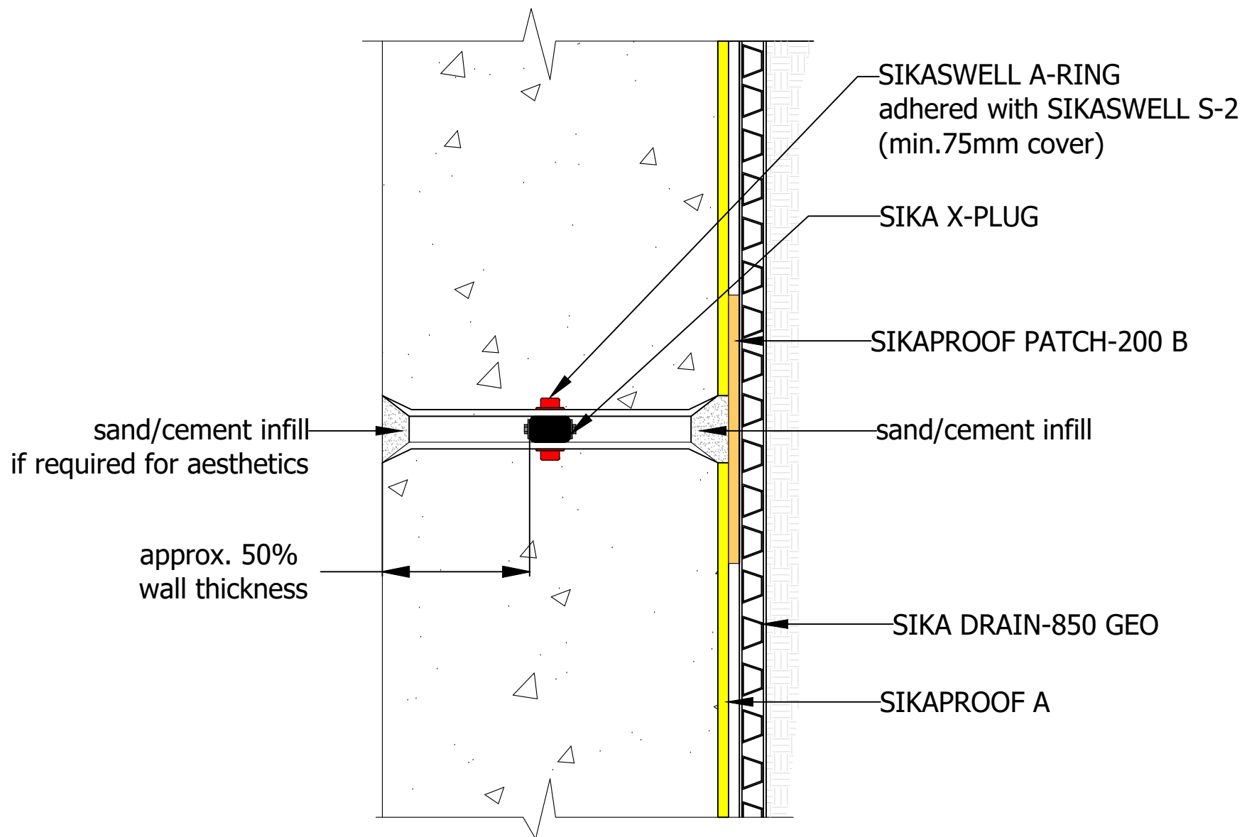
SIKAPROOF A (With Sleeve)
