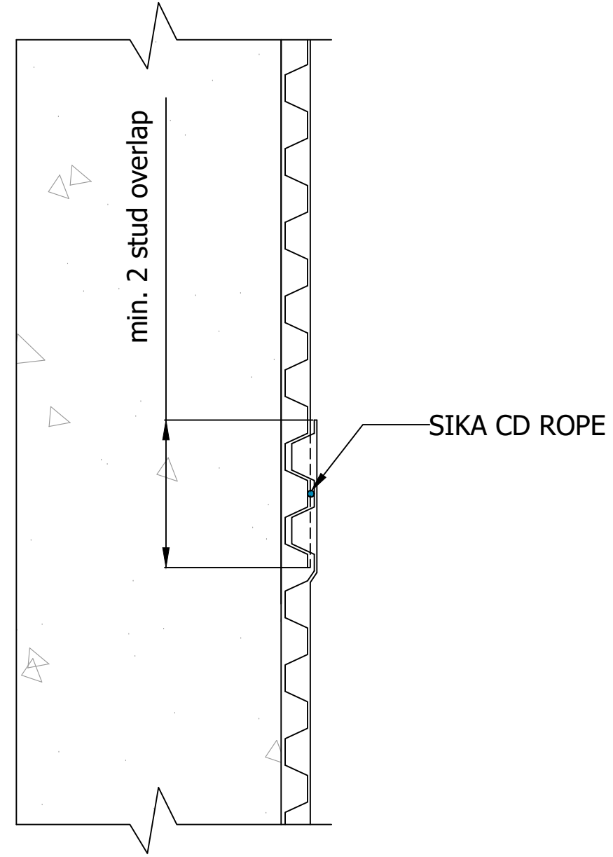
HD20 OVERLAP - VERTICAL APPLICATION
