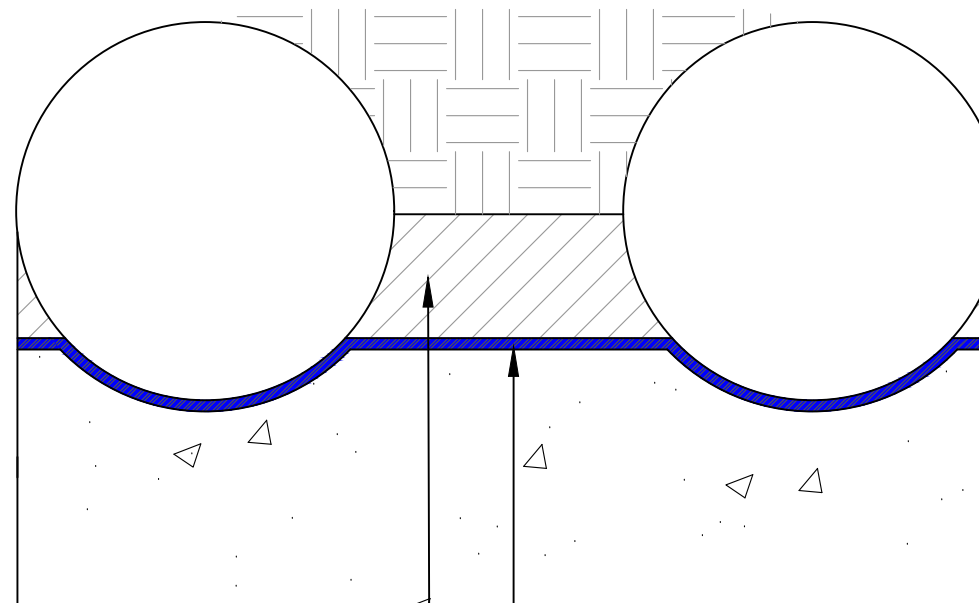
SIKA BENTOSHIELD MAX LM back blinding
