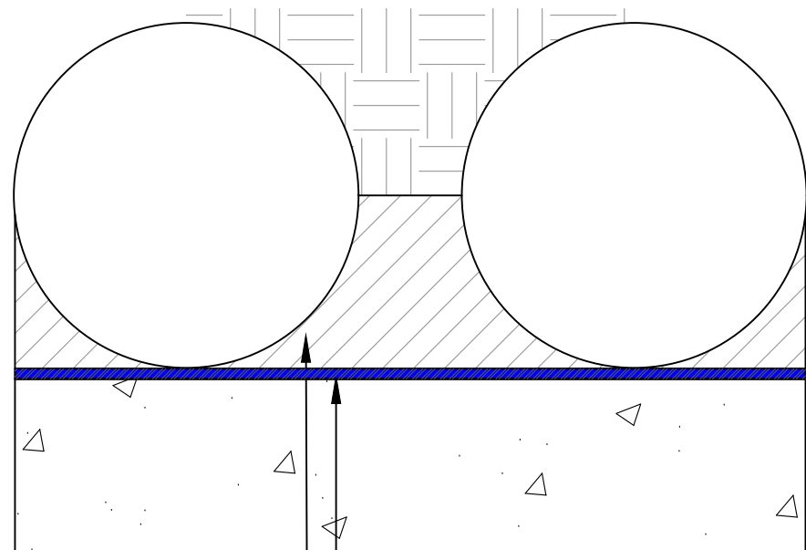
SIKA BENTOSHIELD MAX LM back blinding
